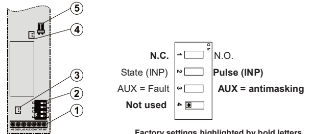
Figure 4 - Transmitter: 1 – terminals, 2 – option DIP switch, 3 – external tamper connector, 4 – external antenna jumper, 5 – external antenna connector
