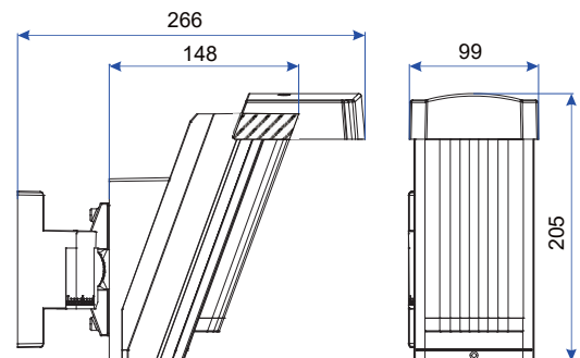
Figure 5: Detector dimensions
